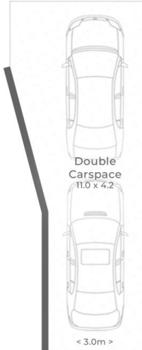
:: CARSPACE Ground Floor
