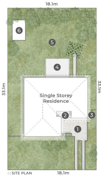
:: SITE PLAN
