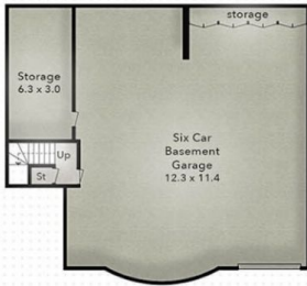
FLOOR PLAN // Lower Floor
