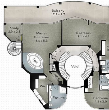
FLOOR PLAN // First Floor
